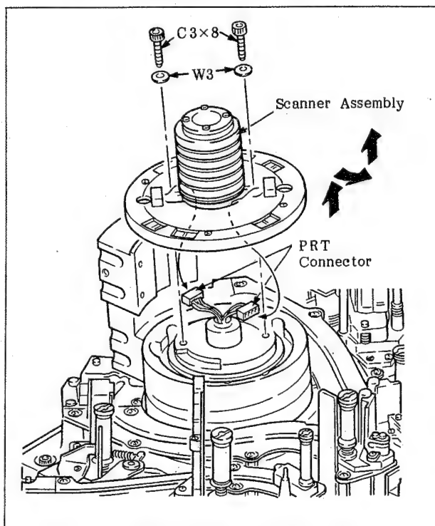
Fig. 6-3 Disassembling the Scanner Assembly
